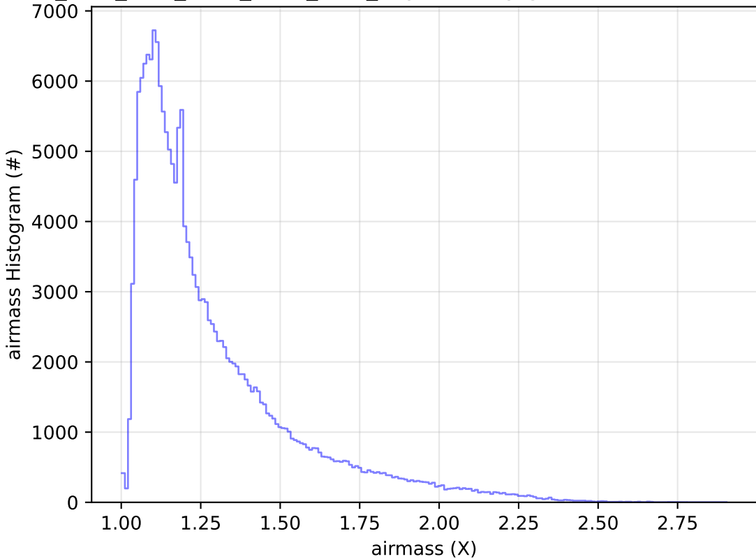
ddf_acor_sf25_lsf30_lsr10_v3.4_10yrs All sky g band: airmass Histogram
