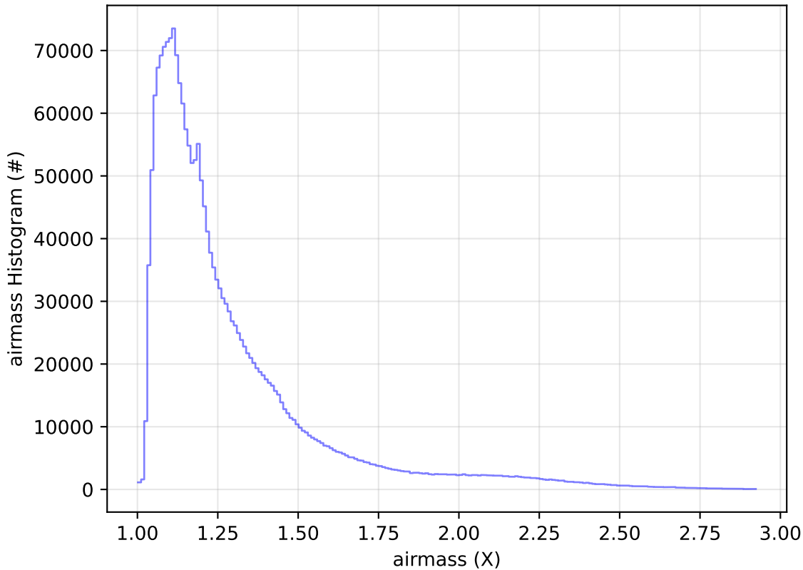
ddf_acor_sf25_lsf30_lsr10_v3.4_10yrs All sky all bands: airmass Histogram
