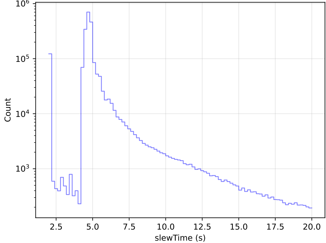
ddf_acor_sf25_Isf30_Isr10_v3.4_10yrs All visits: Zoom Slew Time Histogram
