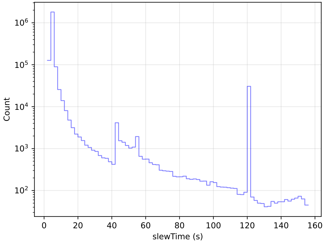
ddf_acor_sf25_lsf30_lsr10_v3.4_10yrs All visits: Slew Time Histogram
