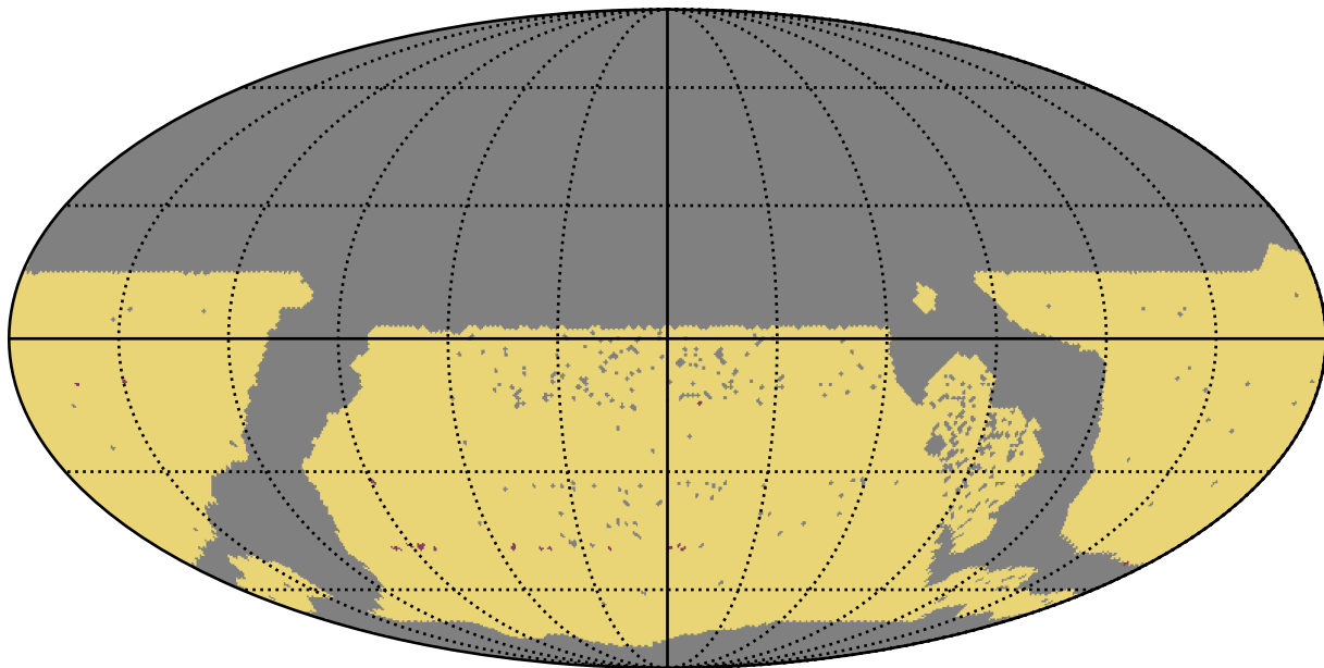
ddf_acor_sf25_lsf30_lsr10_v3.4_10yrs WFD: RapidRevisits
