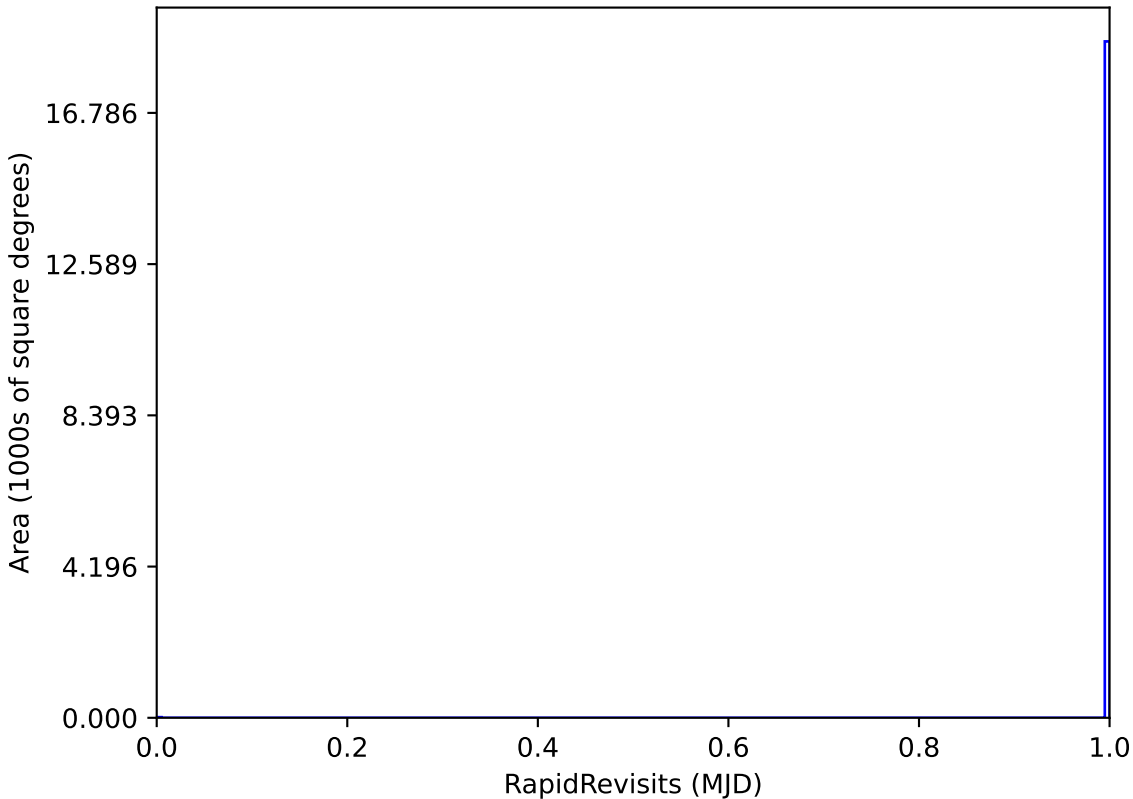
ddf_acor_sf25_lsf30_lsr10_v3.4_10yrs WFD: RapidRevisits
