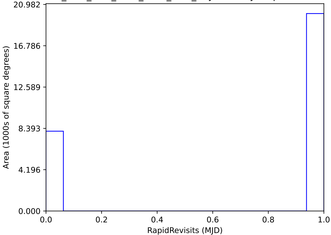
ddf_acor_sf25_lsf30_lsr10_v3.4_10yrs All sky: RapidRevisits
