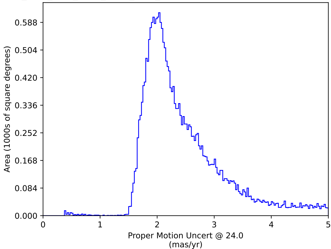
ddf_acor_sf25_lsf30_lsr10_v3.4_10yrs All sky: Proper Motion Uncert @ 24.0
