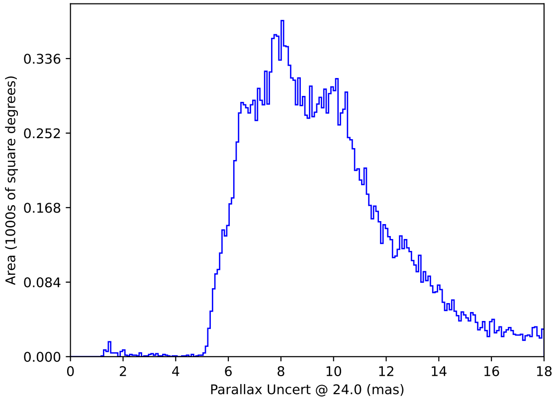
ddf_acor_sf25_lsf30_lsr10_v3.4_10yrs All sky: Parallax Uncert @ 24.0
