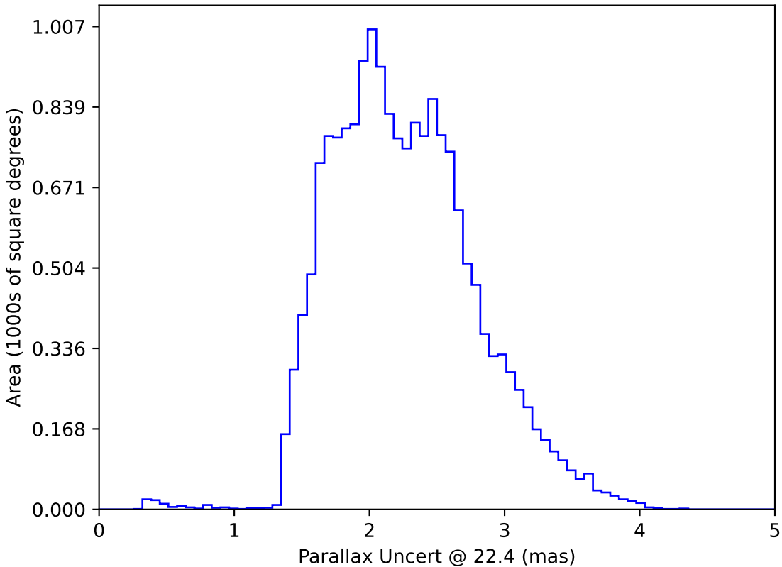
ddf_acor_sf25_lsf30_lsr10_v3.4_10yrs WFD: Parallax Uncert @ 22.4
