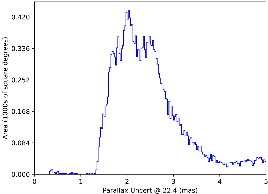
ddf_acor_sf25_lsf30_lsr10_v3.4_10yrs All sky: Parallax Uncert @ 22.4
