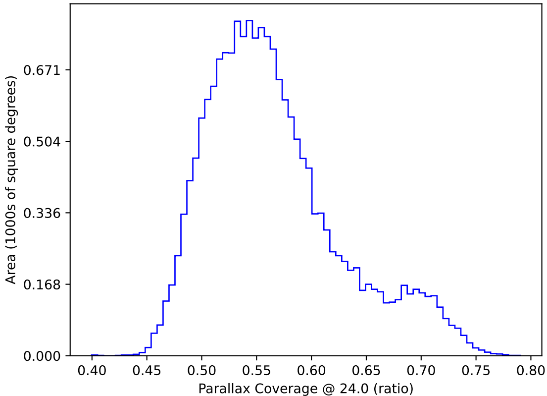
ddf_acor_sf25_lsf30_lsr10_v3.4_10yrs WFD: Parallax Coverage @ 24.0
