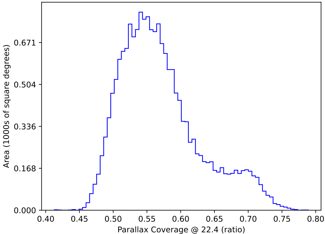
ddf_acor_sf25_lsf30_lsr10_v3.4_10yrs WFD: Parallax Coverage @ 22.4
