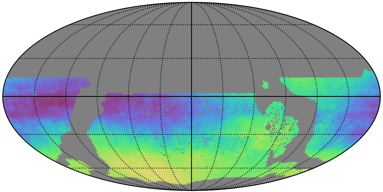
ddf_acor_sf25_lsf30_lsr10_v3.4_10yrs WFD: Parallax-DCR degeneracy @ 24.0
