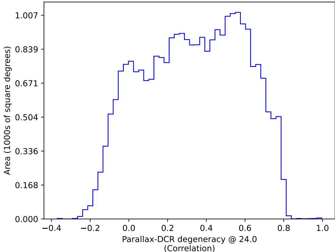
ddf_acor_sf25_lsf30_lsr10_v3.4_10yrs All sky: Parallax-DCR degeneracy @ 24.0
