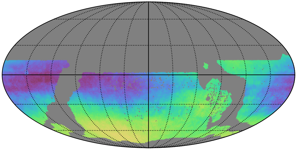
ddf_acor_sf25_lsf30_lsr10_v3.4_10yrs WFD: Parallax-DCR degeneracy @ 22.4
