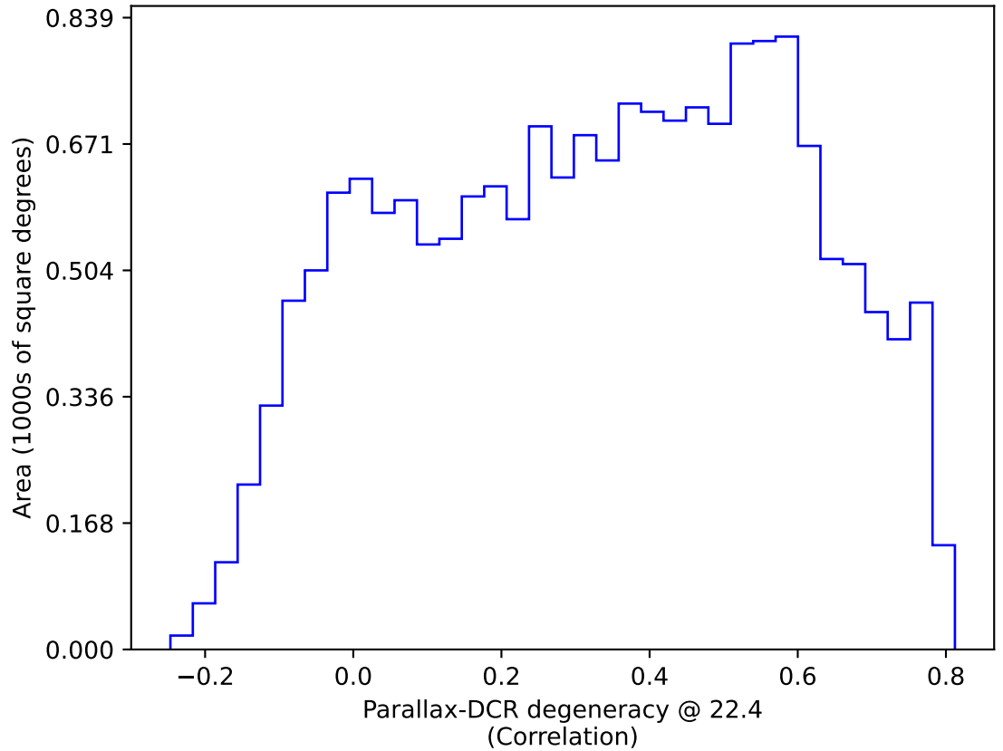
ddf_acor_sf25_lsf30_lsr10_v3.4_10yrs WFD: Parallax-DCR degeneracy @ 22.4
