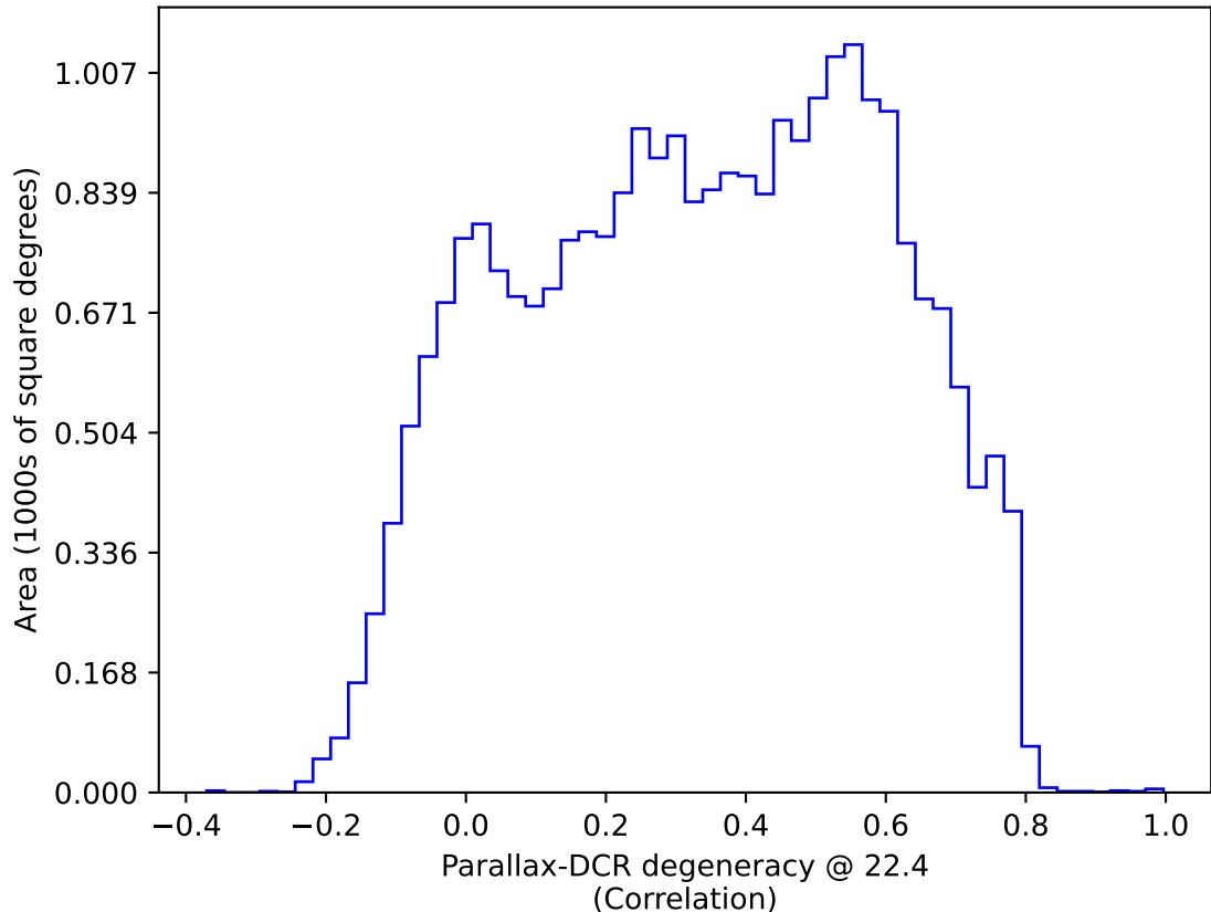
ddf_acor_sf25_lsf30_lsr10_v3.4_10yrs All sky: Parallax-DCR degeneracy @ 22.4
