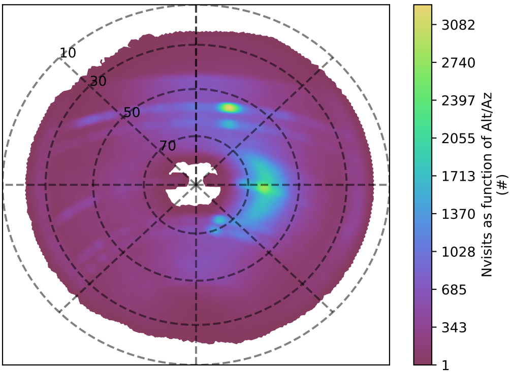
ddf_acor_sf25_lsf30_lsr10_v3.4_10yrs z band: Nvisits as function of Alt/Az
