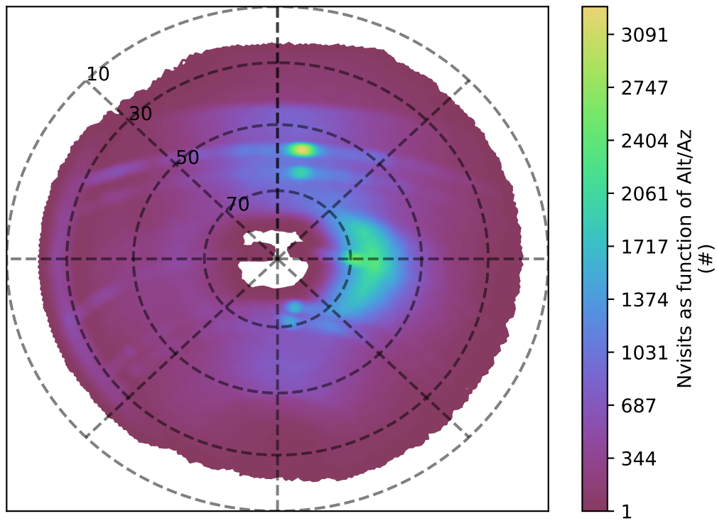
ddf_acor_sf25_lsf30_lsr10_v3.4_10yrs r band: Nvisits as function of Alt/Az
