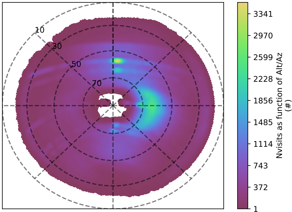
ddf_acor_sf25_lsf30_lsr10_v3.4_10yrs i band: Nvisits as function of Alt/Az
