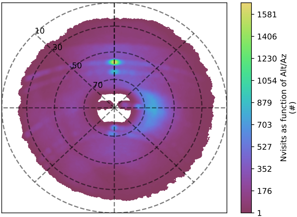
ddf_acor_sf25_lsf30_lsr10_v3.4_10yrs g band: Nvisits as function of Alt/Az
