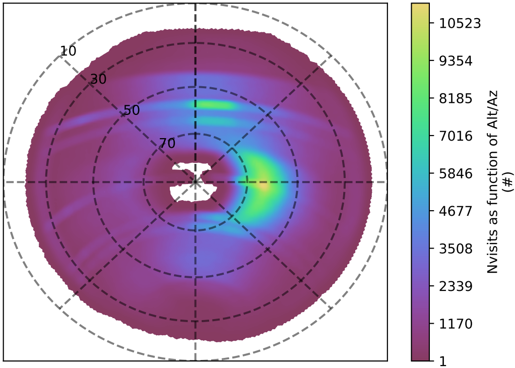
ddf_acor_sf25_lsf30_lsr10_v3.4_10yrs all bands: Nvisits as function of Alt/Az
