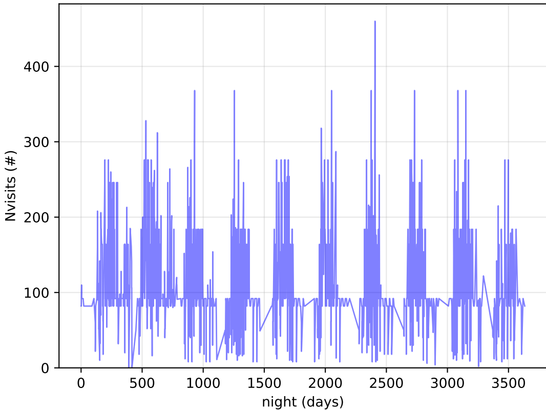
ddf_acor_sf25_ls30_lsr10_v3.4_10yrs DDF: Nvisits
