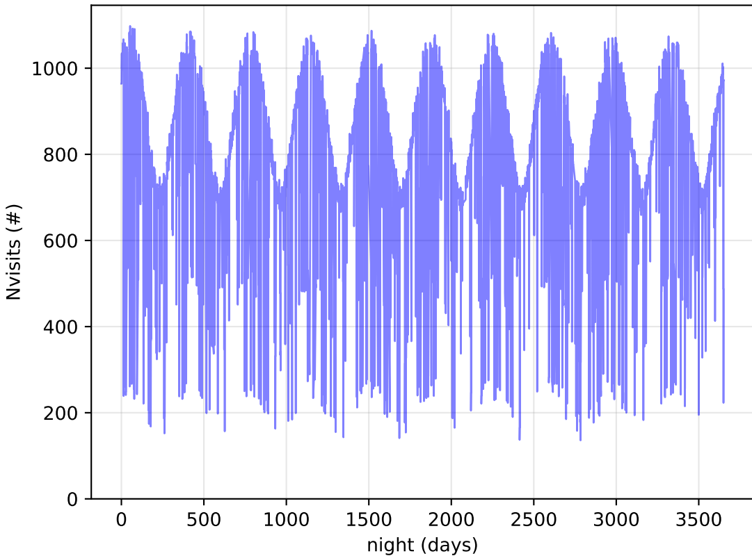
ddf_acor_sf25_lsf30_lsr10_v3.4_10yrs All visits: Nvisits
