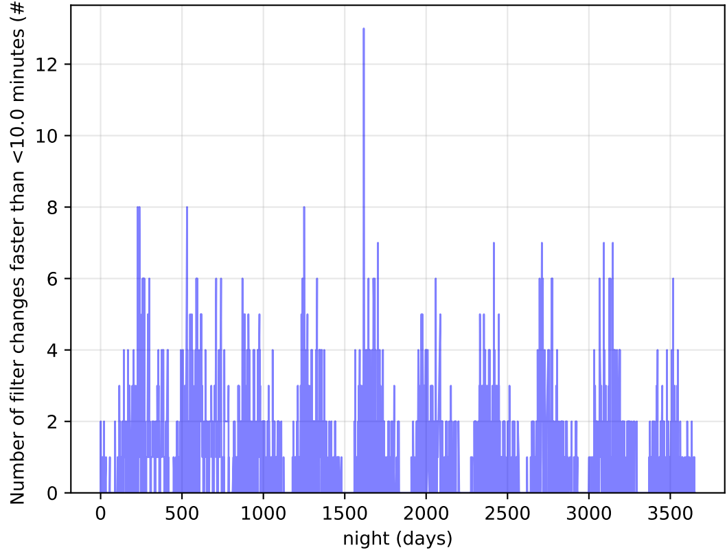
ddf_acor_sf25_Isf30_Isr10_v3.4_10yrs Per Night: Number of filter changes faster than <10.0 minutes
