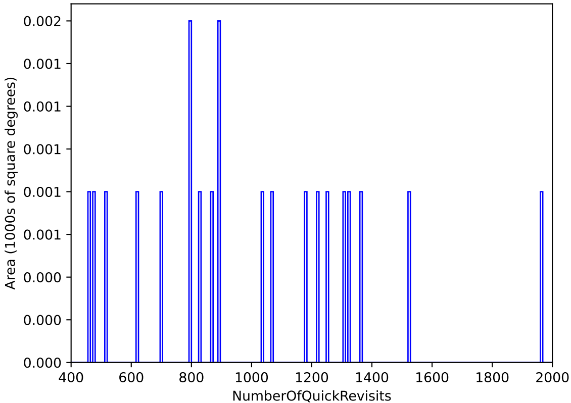
ddf_acor_sf25_lsf30_lsr10_v3.4_10yrs WFD: NumberOfQuickRevisits
