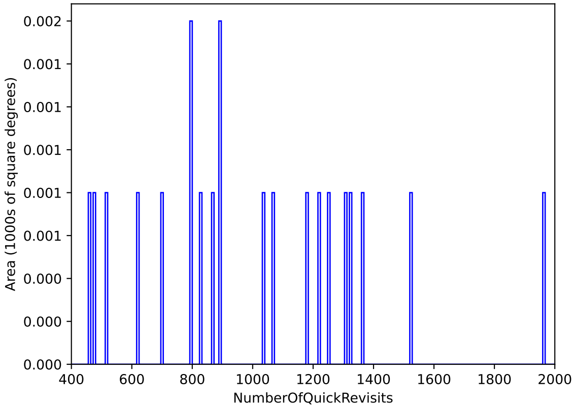
ddf_acor_sf25_lsf30_lsr10_v3.4_10yrs All sky: NumberOfQuickRevisits
