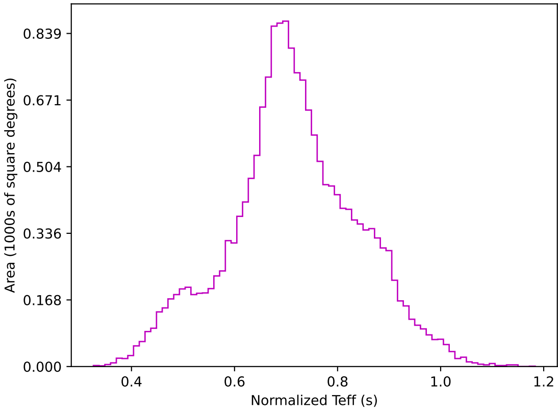
ddf_acor_sf25_lsf30_lsr10_v3.4_10yrs WFD z band: Normalized Teff
