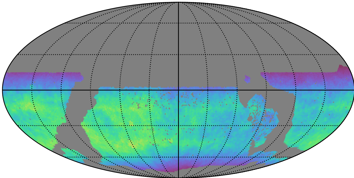
ddf_acor_sf25_lsf30_lsr10_v3.4_10yrs WFD y band: Normalized Teff
