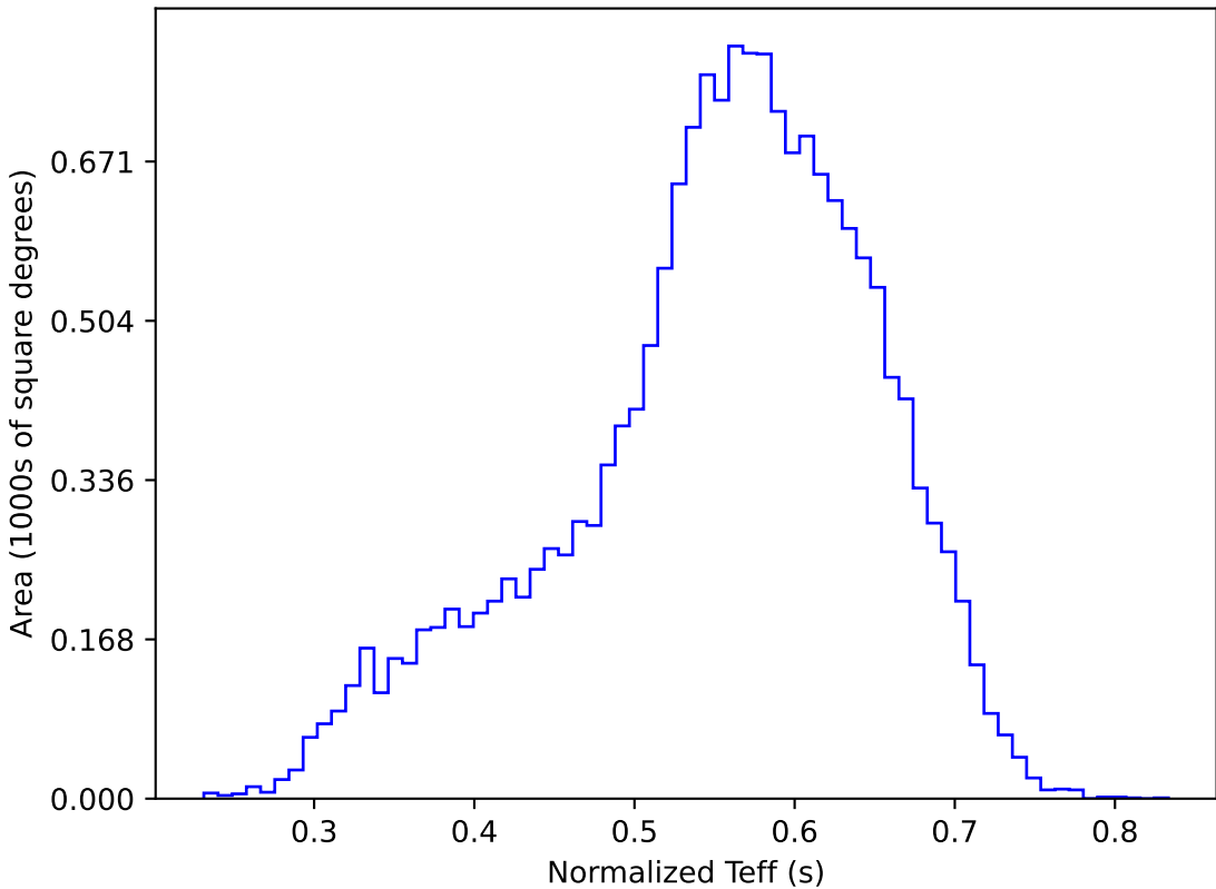
ddf_acor_sf25_lsf30_lsr10_v3.4_10yrs WFD y band: Normalized Teff
