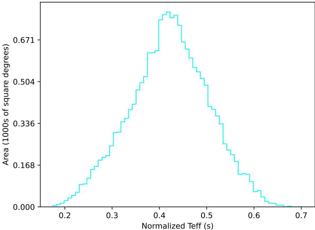
ddf_acor_sf25_lsf30_lsr10_v3.4_10yrs WFD u band: Normalized Teff
