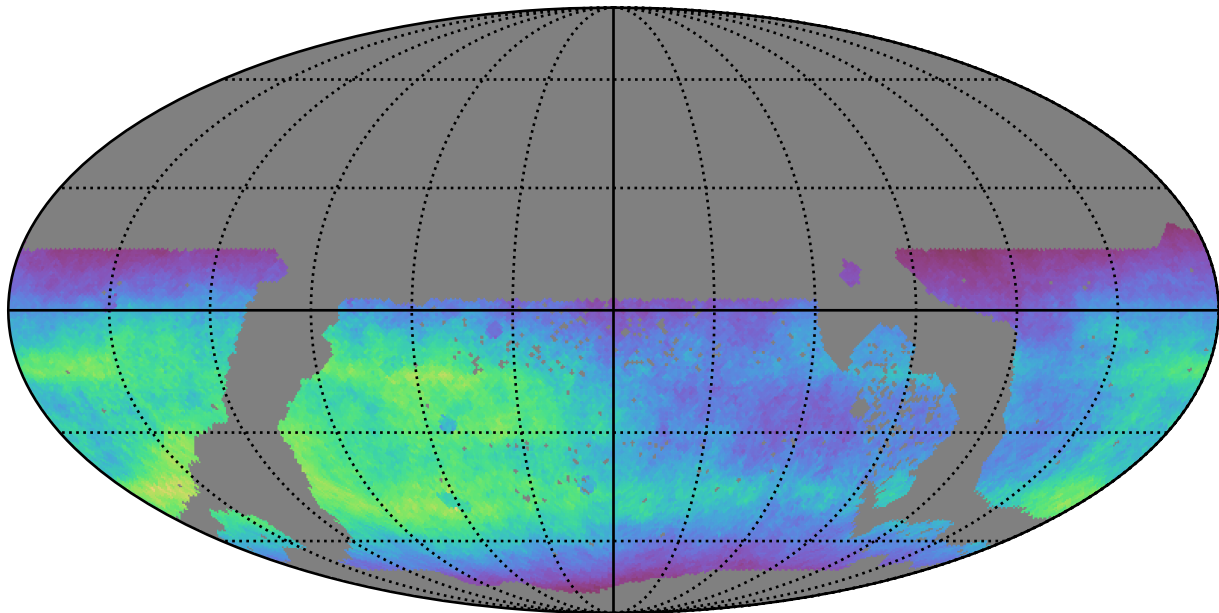
ddf_acor_sf25_lsf30_lsr10_v3.4_10yrs WFD r band: Normalized Teff
