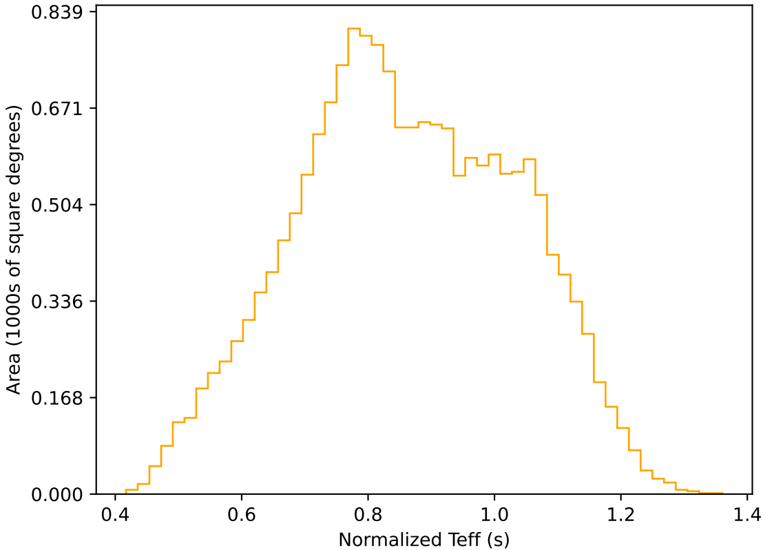
ddf_acor_sf25_lsf30_lsr10_v3.4_10yrs WFD r band: Normalized Teff
