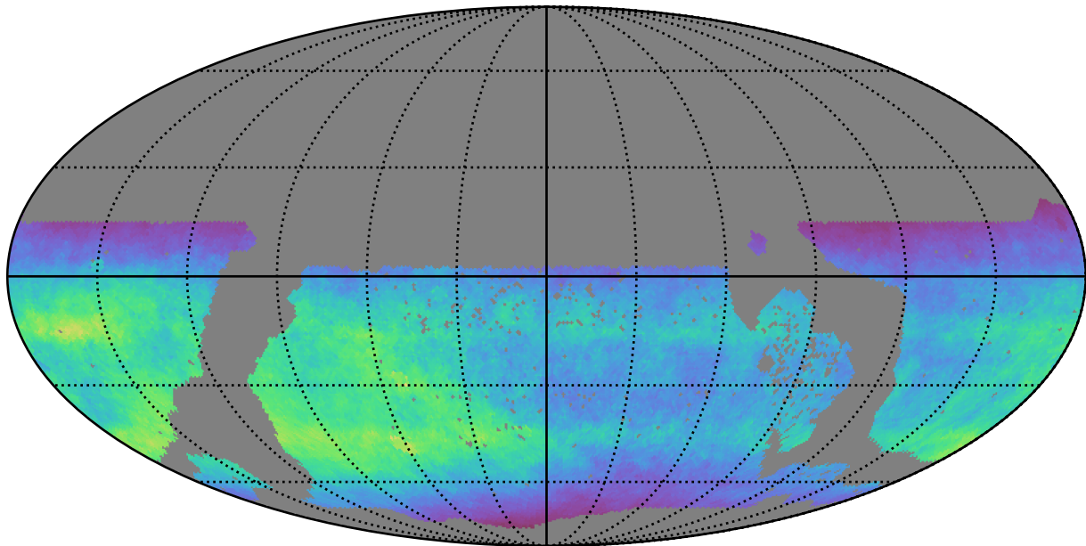
ddf_acor_sf25_lsf30_lsr10_v3.4_10yrs WFD i band: Normalized Teff
