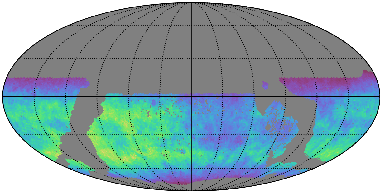
ddf_acor_sf25_lsf30_lsr10_v3.4_10yrs WFD g band: Normalized Teff
