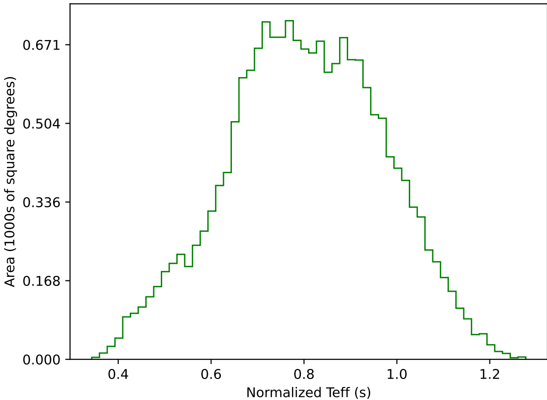
ddf_acor_sf25_lsf30_lsr10_v3.4_10yrs WFD g band: Normalized Teff
