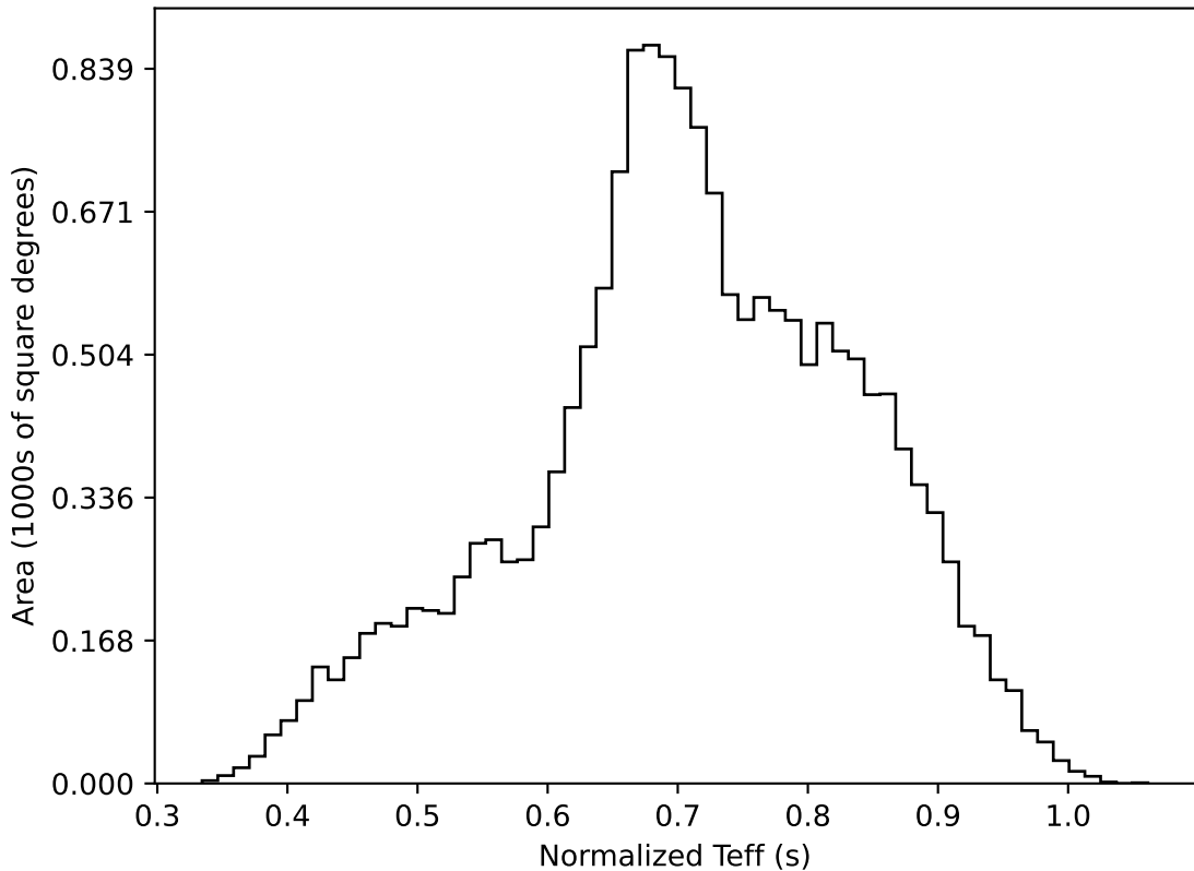
ddf_acor_sf25_lsf30_lsr10_v3.4_10yrs WFD all bands: Normalized Teff
