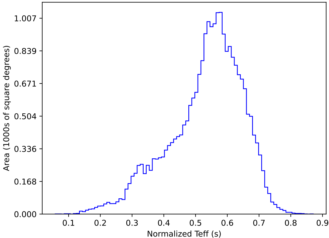
ddf_acor_sf25_lsf30_lsr10_v3.4_10yrs All sky y band: Normalized Teff
