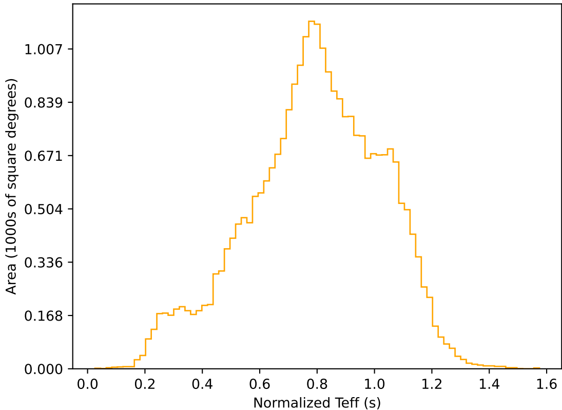
ddf_acor_sf25_lsf30_lsr10_v3.4_10yrs All sky r band: Normalized Teff
