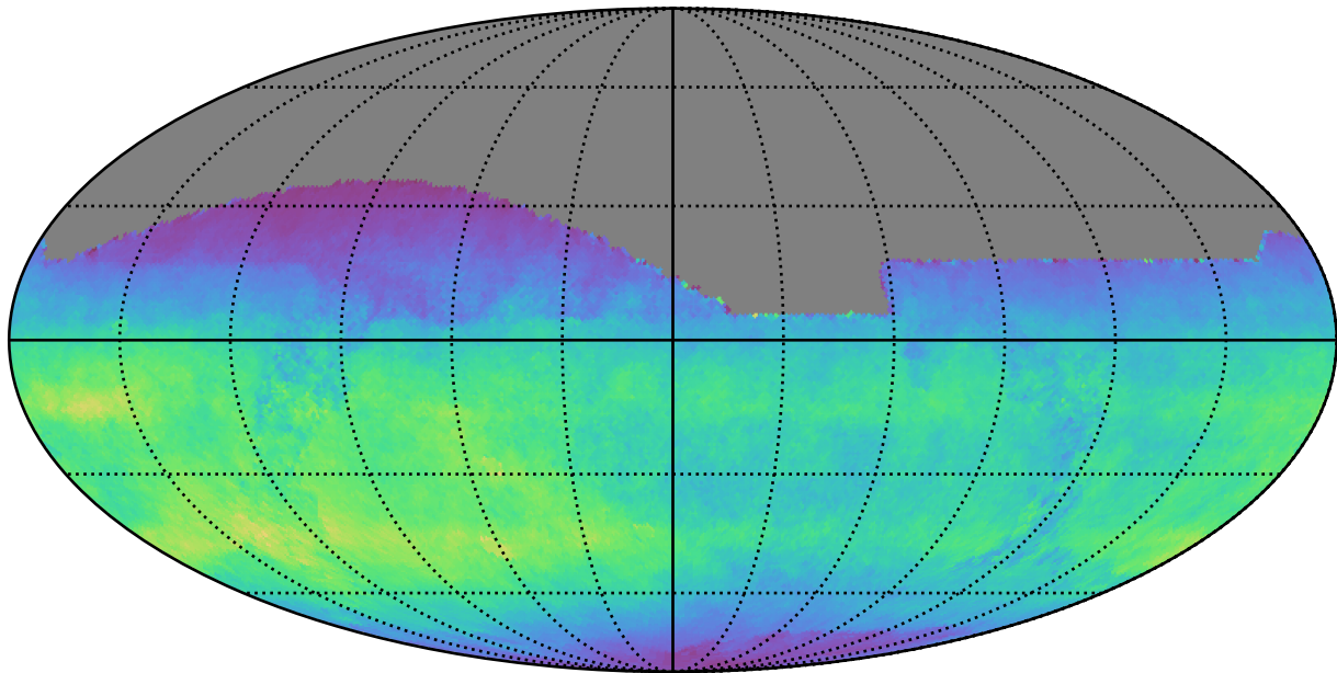
ddf_acor_sf25_lsf30_lsr10_v3.4_10yrs All sky i band: Normalized Teff
