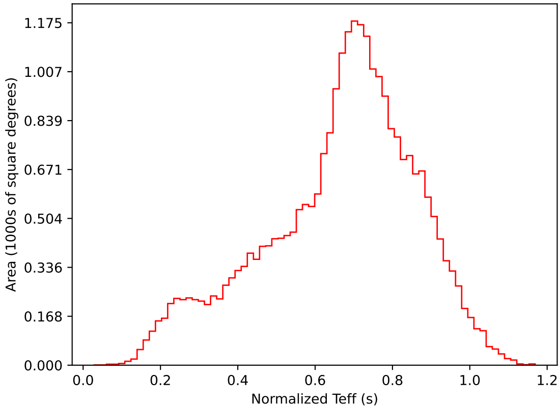
ddf_acor_sf25_lsf30_lsr10_v3.4_10yrs All sky i band: Normalized Teff
