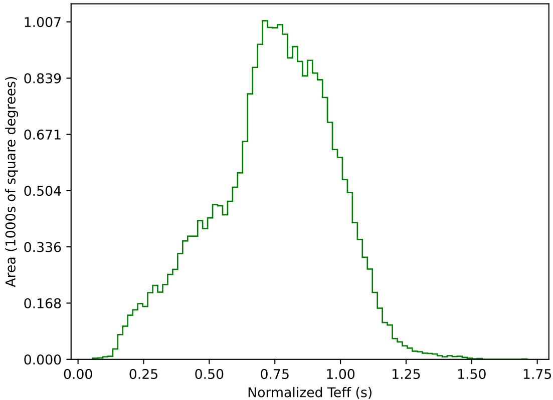
ddf_acor_sf25_lsf30_lsr10_v3.4_10yrs All sky g band: Normalized Teff
