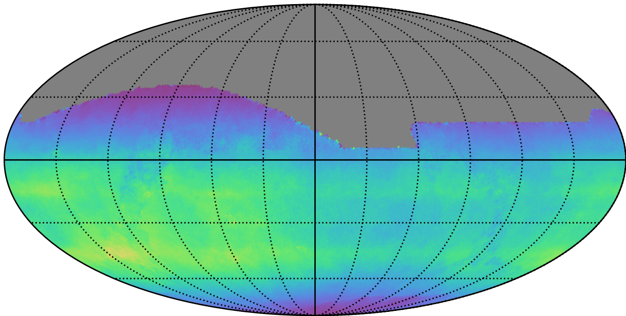
ddf_acor_sf25_lsf30_lsr10_v3.4_10yrs All sky all bands: Normalized Teff
