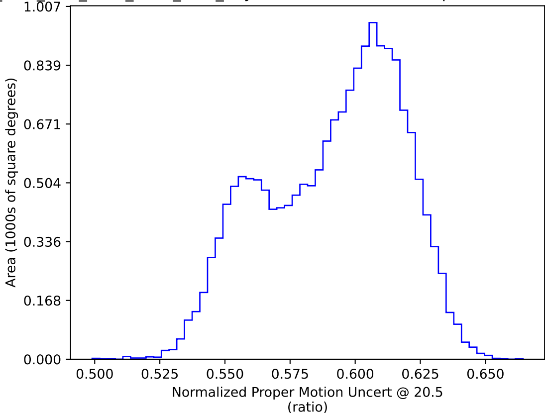
ddf_acor_sf25_lsf30_lsr10_v3.4_10yrs WFD: Normalized Proper Motion Uncert @ 20.5
