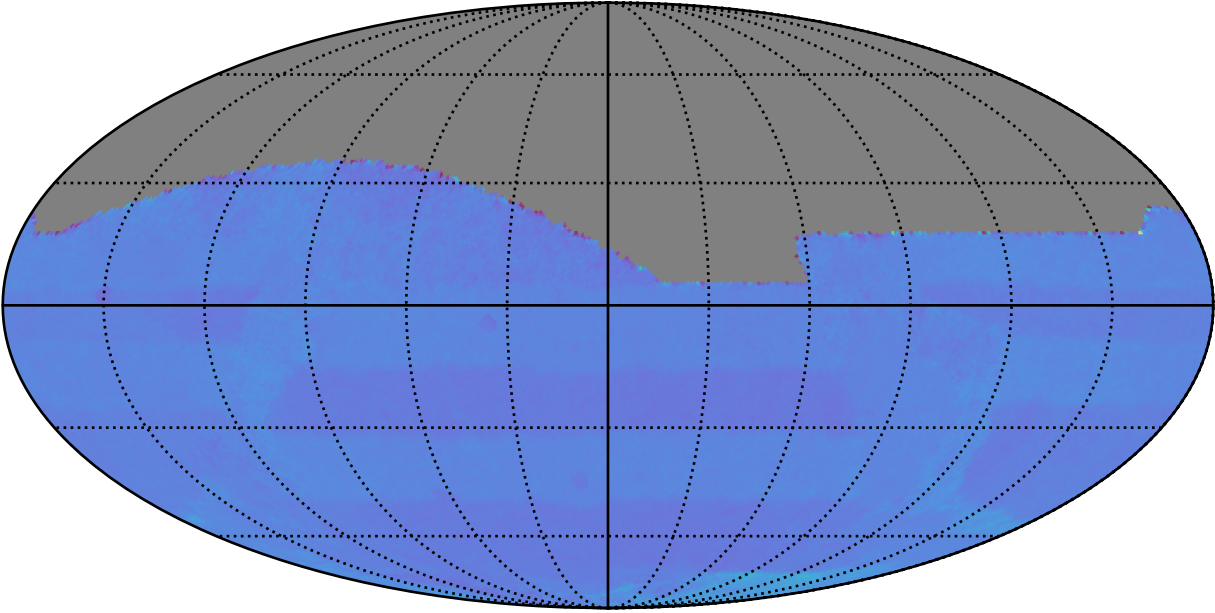
ddf_acor_sf25_lsf30_lsr10_v3.4_10yrs All sky: Normalized Proper Motion Uncert @ 20.5
