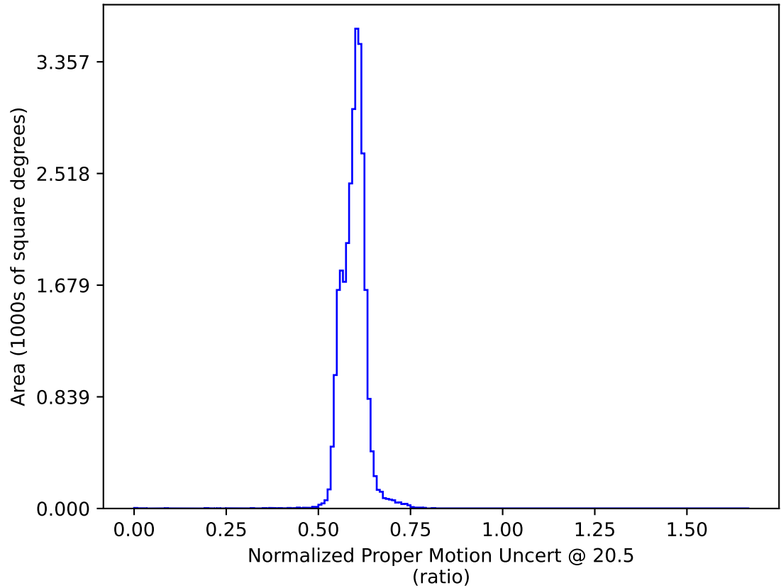
ddf_acor_sf25_lsf30_lsr10_v3.4_10yrs All sky: Normalized Proper Motion Uncert @ 20.5
