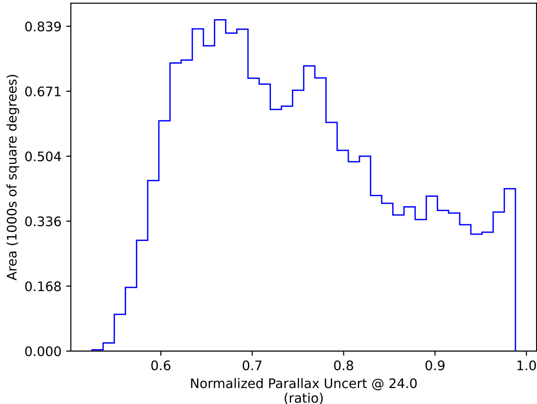
ddf_acor_sf25_lsf30_lsr10_v3.4_10yrs WFD: Normalized Parallax Uncert @ 24.0
