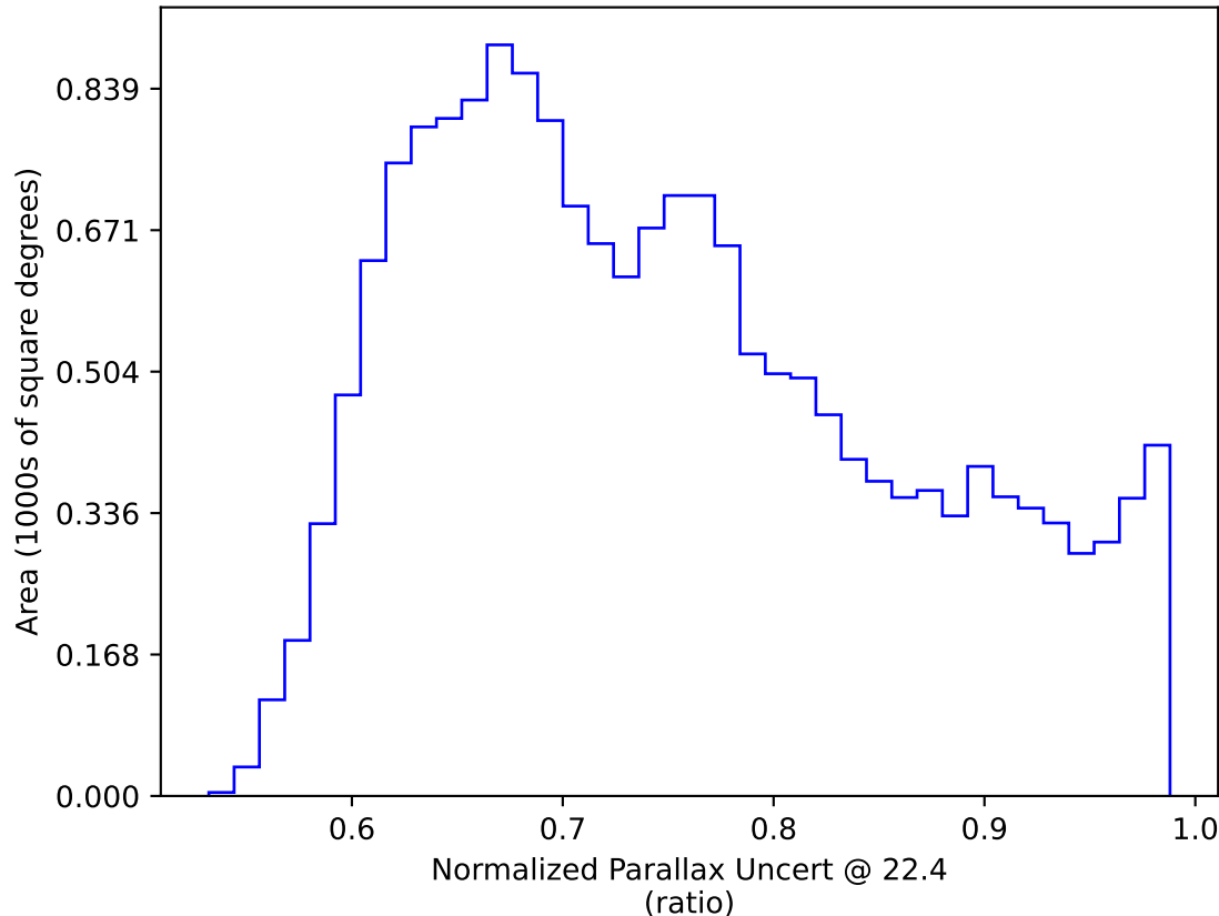
ddf_acor_sf25_lsf30_lsr10_v3.4_10yrs WFD: Normalized Parallax Uncert @ 22.4
