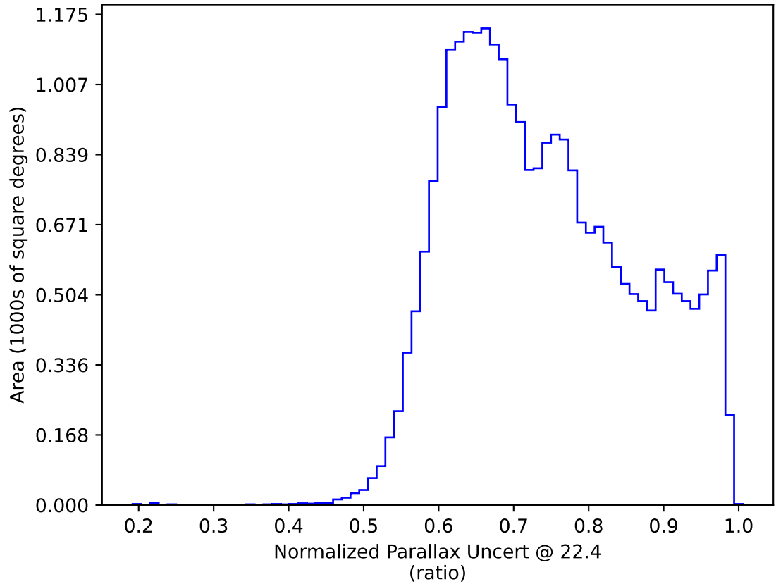
ddf_acor_sf25_lsf30_lsr10_v3.4_10yrs All sky: Normalized Parallax Uncert @ 22.4
